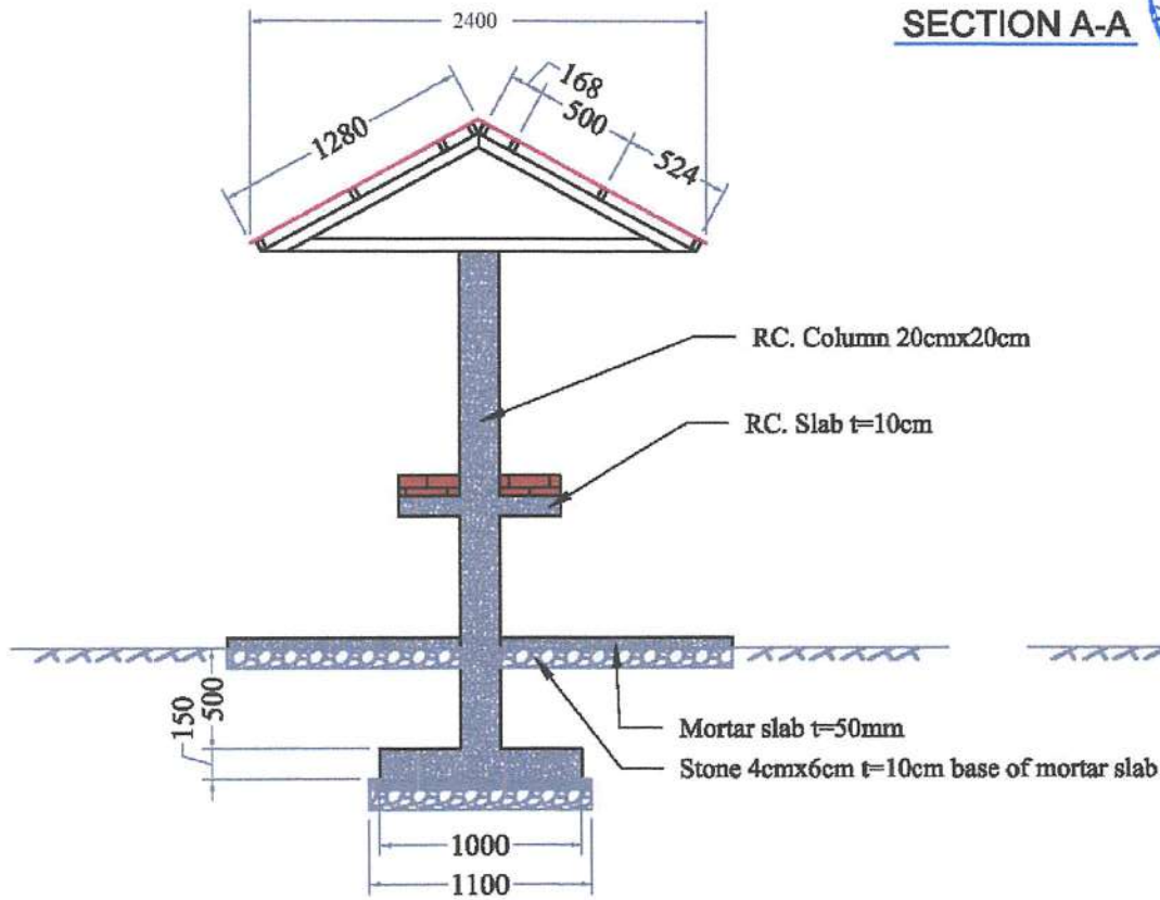
SECTION COLUMN
