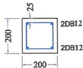
SECTION COLUMN
