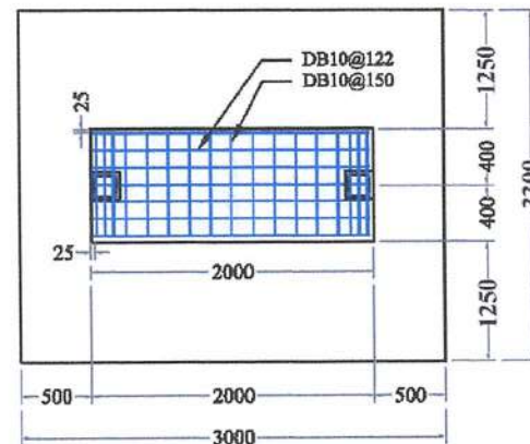
REINFORCEMENT OF SECTION B-B
