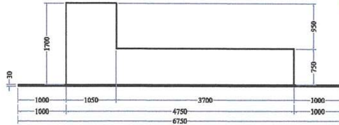
VIEW A
